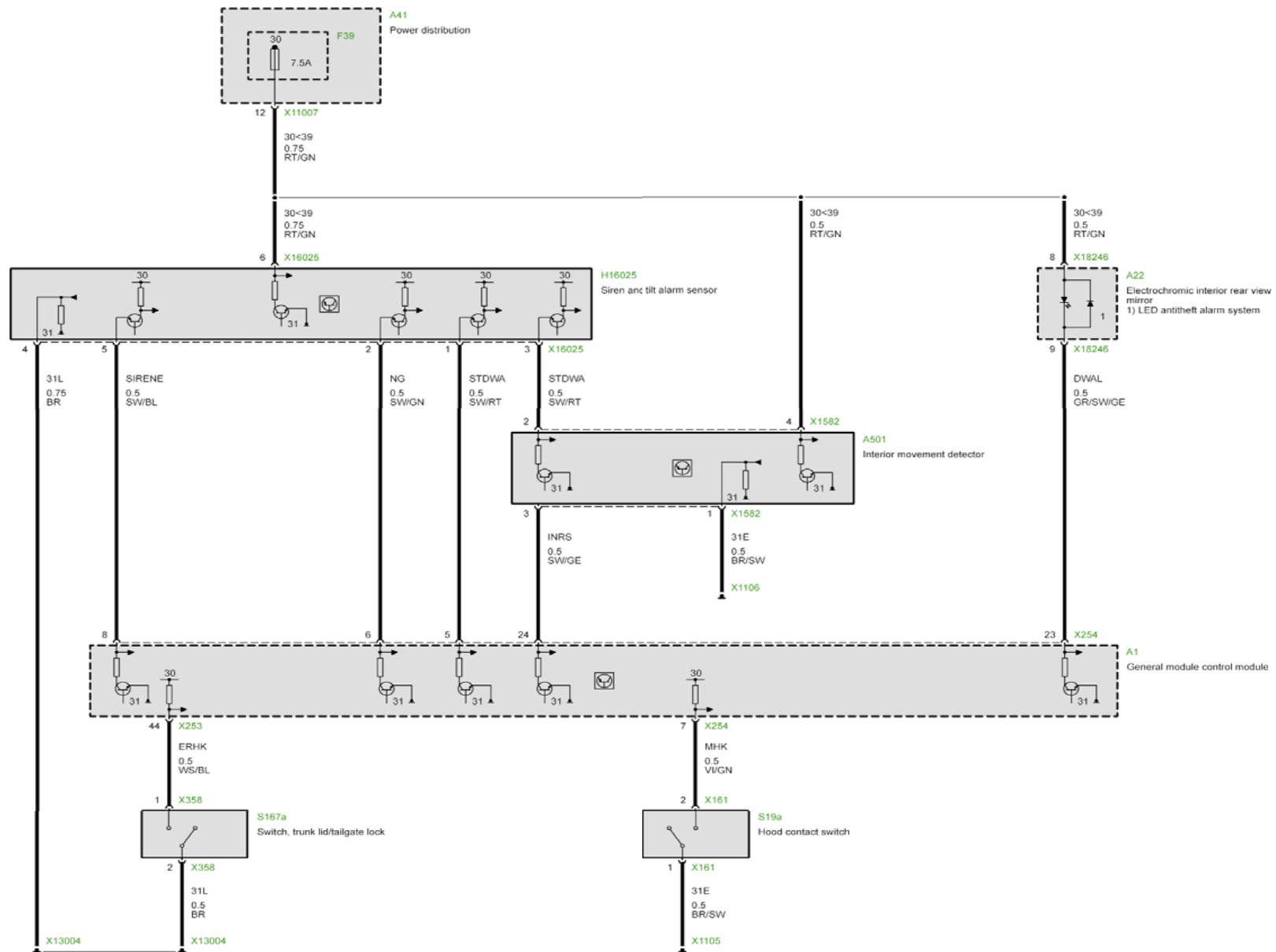
E85 E86 Antitheft alarm system
