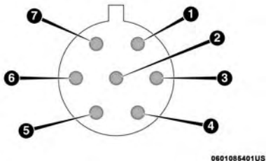
Seven-Pin Connector
